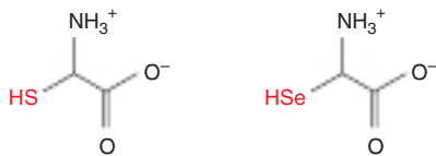
FIGURE 3–1 Cysteine (left) and selenocysteine (right). pK_3 for the selenyl proton of selenocysteine is 5.2. Since this is 3 pH units lower than that of cysteine, selenocysteine represents a better nucleophile at or below pH 7.4.
